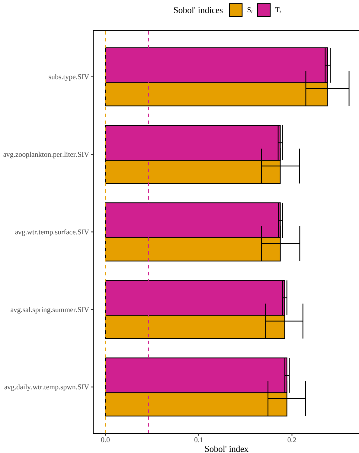
Figure 4. Results of a sensitivity analysis for the alewifeJuvAndSAEL model based on an arithmetic mean structure. Dashed lines represent baseline numerical approximation error for S_i and T_i ( i.e. , dummy variables).
