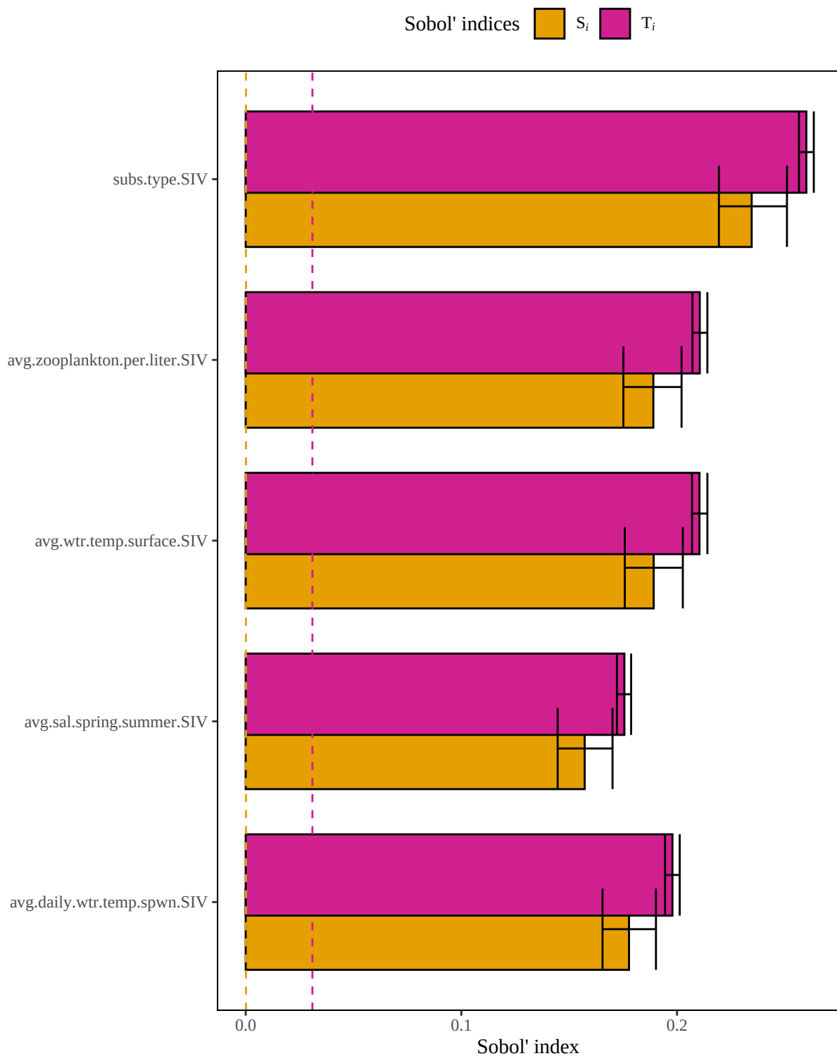
Figure 5. Results of a sensitivity analysis for the alewifeJuvAndSAEL model based on a geometric mean structure. Dashed lines represent baseline numerical approximation error for S_i and T_i ( i.e. , dummy variables).
